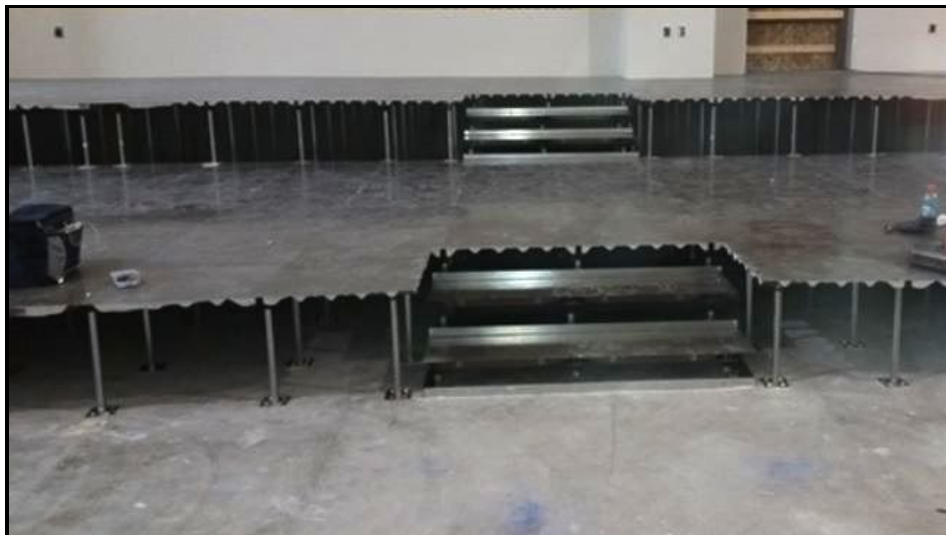
Construction of a tiered classroom for a corporate headquarters in Findlay, OH
